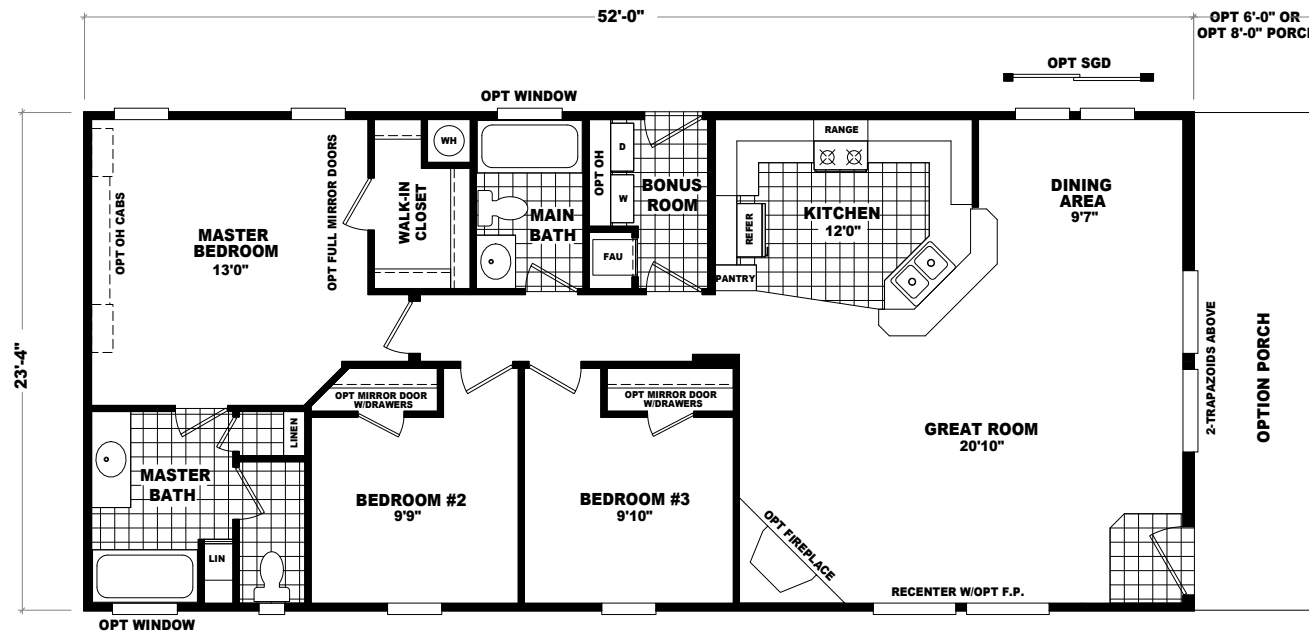
MODEL: 2452A-96 APPROXIMATELY 1213 SQ. FT. 3 BEDROOM, 2 BATH
